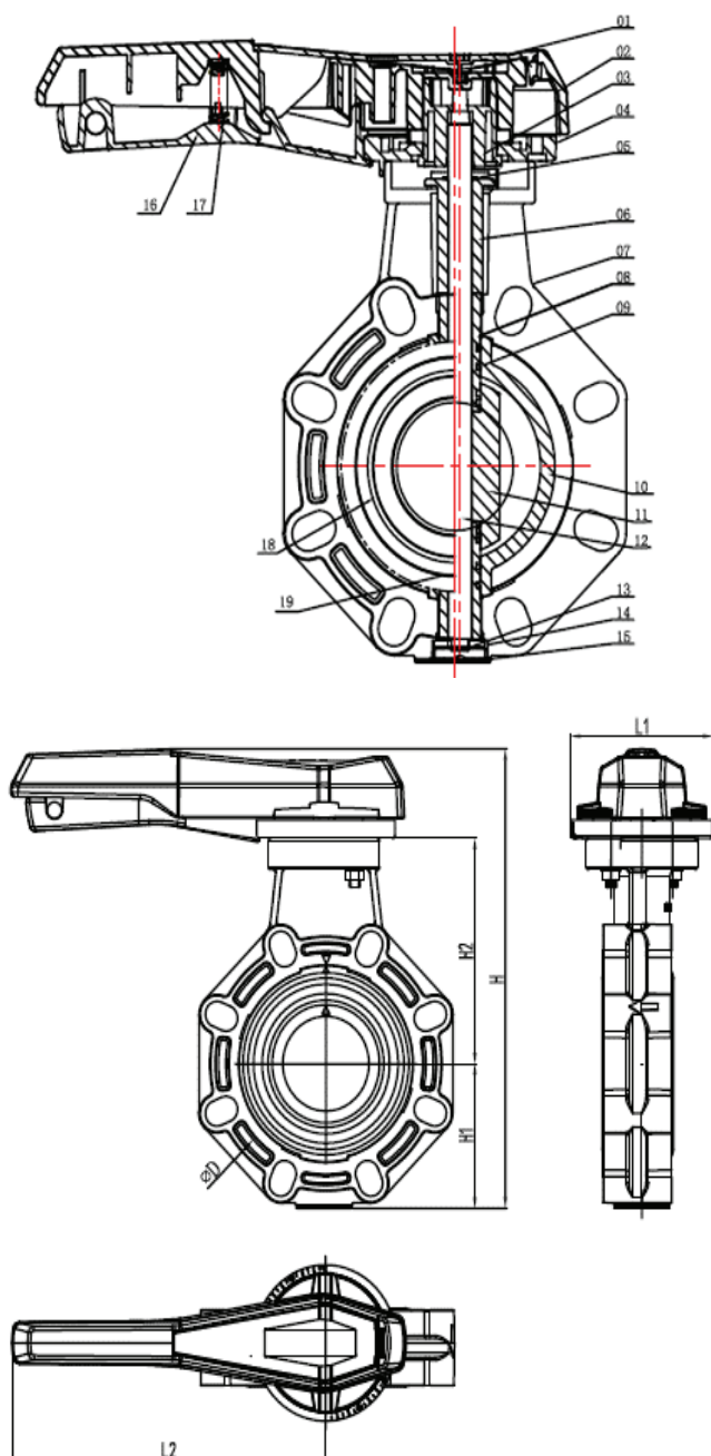
Handled Butterfly Valve, PVC-U/C (ASTM)
