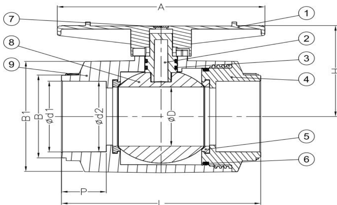
CTS SUPER COMPACT BALL VALVE DN15 - DN25
